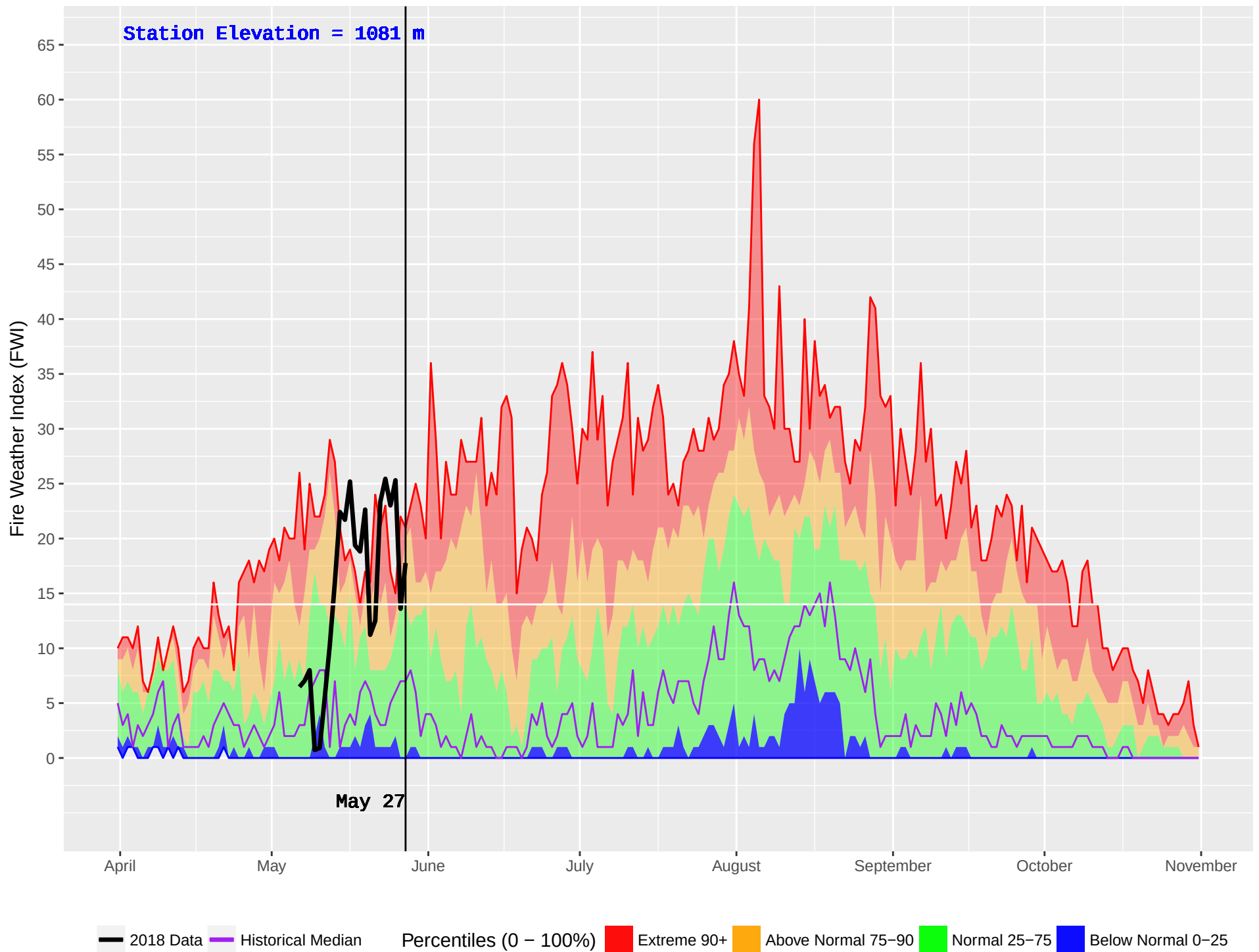
GAVIN (227) : Historical (1981–2016) and Current (2018) Noon Fire Weather Index (FWI)
