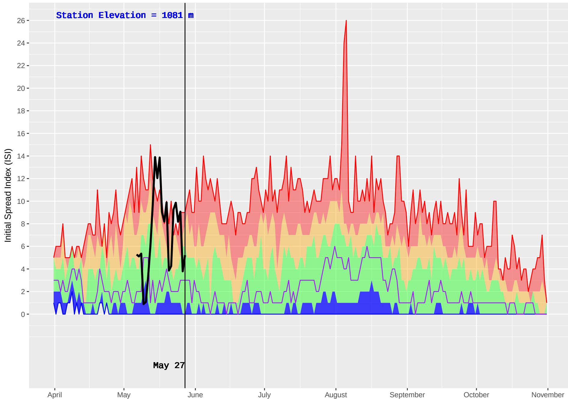
GAVIN (227) : Historical (1981–2016) and Current (2018) Noon Initial Spread Index (ISI)
