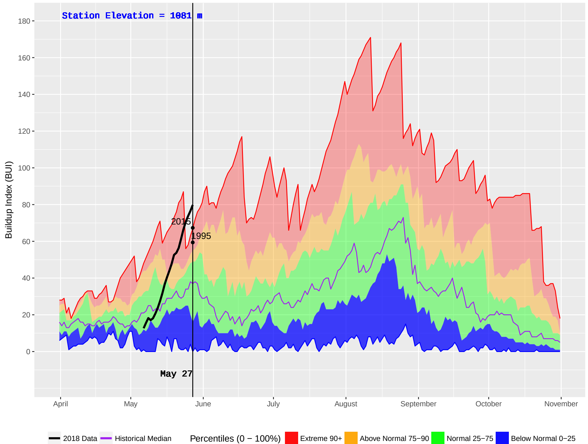
GAVIN (227) : Historical (1981–2016) and Current (2018) Noon Buildup Index (BUI)
